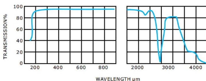
Transmission Curve Sapphire
